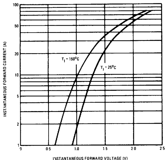
Fig. 7 - Maximum Instantaneous Forward Voltage Vs. Instantaneous Forward Current
