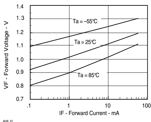
Figure 1. Forward Voltage vs. Forward Current
