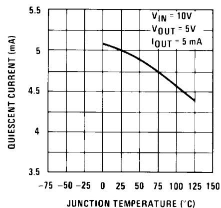
Quiescent Current
