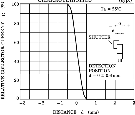
DETECTION POSITION CHARACTERISTICS (typ.)
