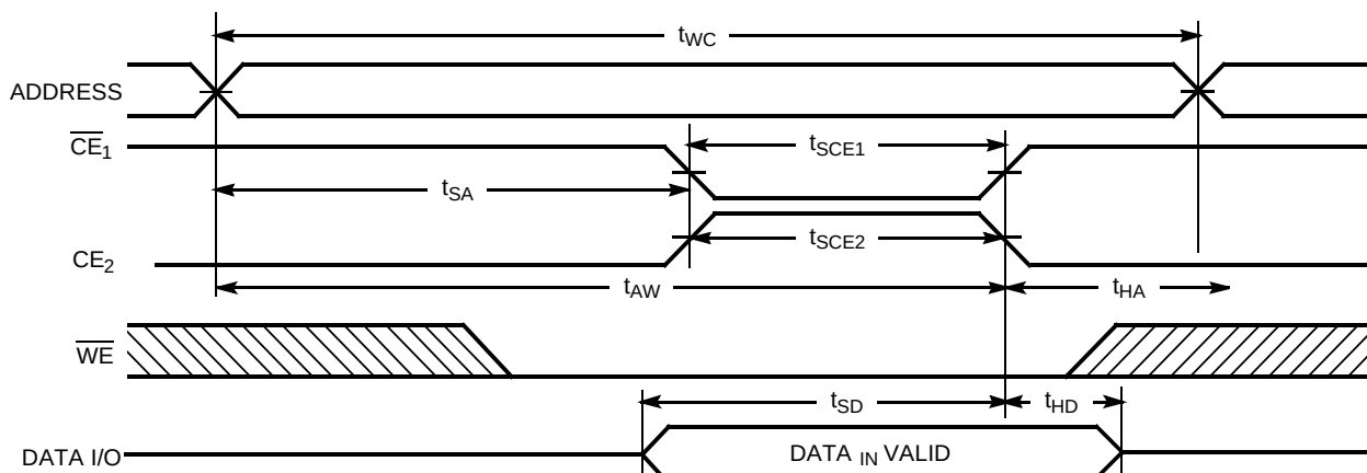
Write Cycle No. 2 ( \overline{\text{CE}} Controlled) [13,14,15]
