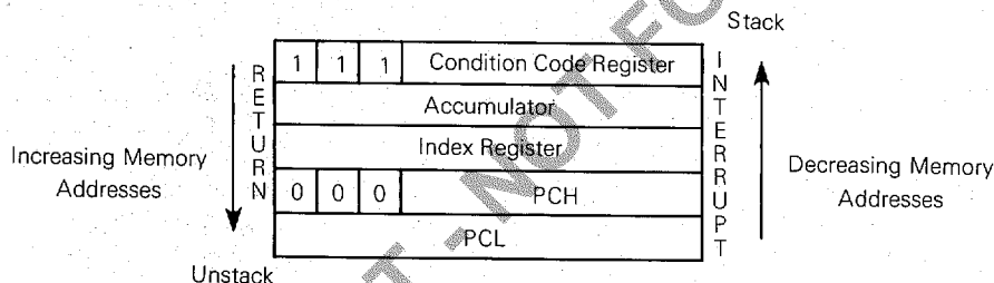
FIGURE 14 — STACKING ORDER
